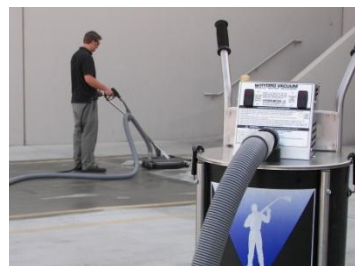
The PVR is an excellent vacuum source for the Twister Vac accessory to recycle the wash water as the twister is cleaning.
