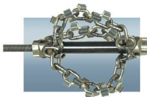
FR-3-4HDCK 3" – 4" Heavy Duty Carbide Tipped Chain Cutter – Triple Chain – For Roots and Descaling
