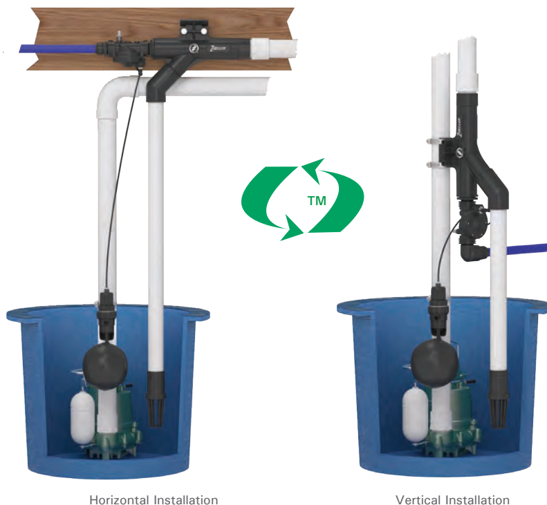
Horizontal Installation
