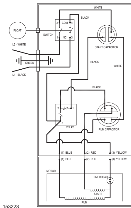
WIRING DIAGRAM FOR MODELS "M803", "M805", "M807", "N803", "N805", "N807", "D803", "D805", "D807", "DH803", "DH805", "DH807" 4/15 thru Current
