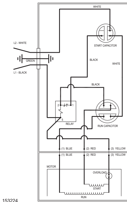
WIRING DIAGRAM FOR MODELS "N803", "N805", "N807", "E803", "E805", "E807", "EI803", "EI805", "EI807", "DH803", "DH805", "DH807" 4/15 thru Current
