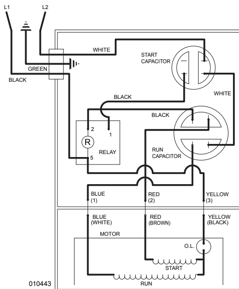
WIRING DIAGRAM FOR MODELS "N818", "E818", "EI818", "I818" All Revisions
