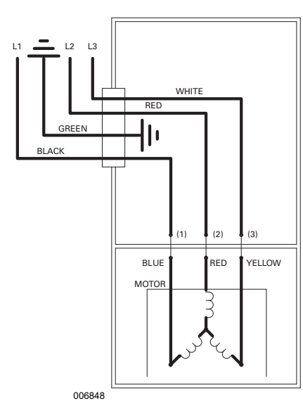
WIRING DIAGRAM FOR MODELS "J818", "F818", "G818", and "BA818" All Revisions 09/17 thru 10/23
