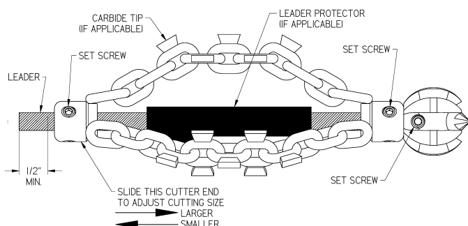
ATTACHING ADJUSTABLE CHAIN CUTTERS & CLOGCHOPPER COMBINATION TO A LEADER
