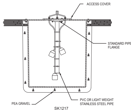
TYPICAL FLOAT HANGER ON STEEL COVER PITS
